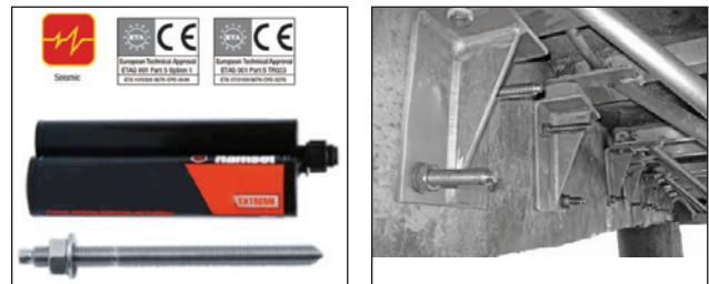
Figure 1 Heavy duty chemical anchor
