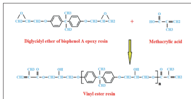
Figure 3 Example of a vinyl ester chemical formulation
