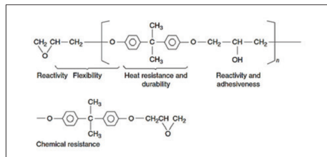
Figure 2 Example of an epoxy chemical formulation
