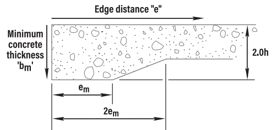
CONCRETE THICKNESS
